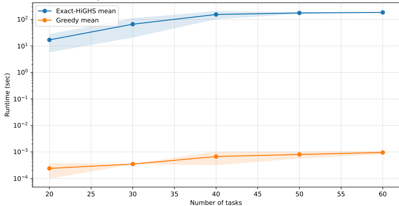
Computational runtime across scaled TTAP instances - 6 Helos / 7 Areas
